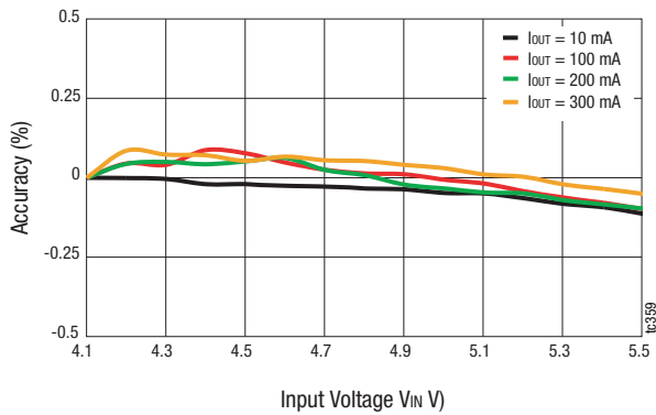
Figure 21. Buck 2 Line Regulation (VOUT = 1.8 V)
