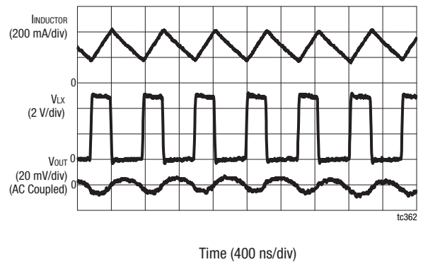
Figure 24. Buck 2 Output Ripple (VIN = 5.0 V, VOUT = 1.8 V, COUT = 4.7 μF, 300 mA Load)
