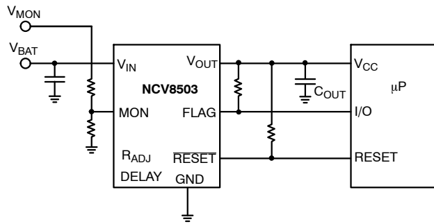
Figure 18. Flag/Monitor Function
