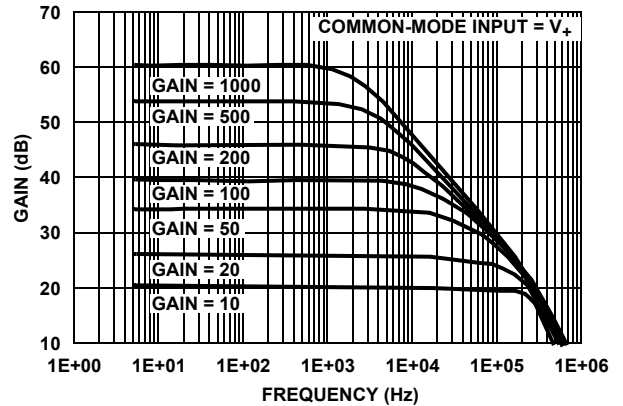
FIGURE 2. ISL28273 FREQUENCY RESPONSE vs CLOSED LOOP GAIN, V_{CM} = V_+ = 5V
