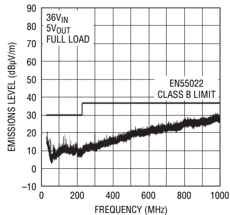
Radiated Emissions
