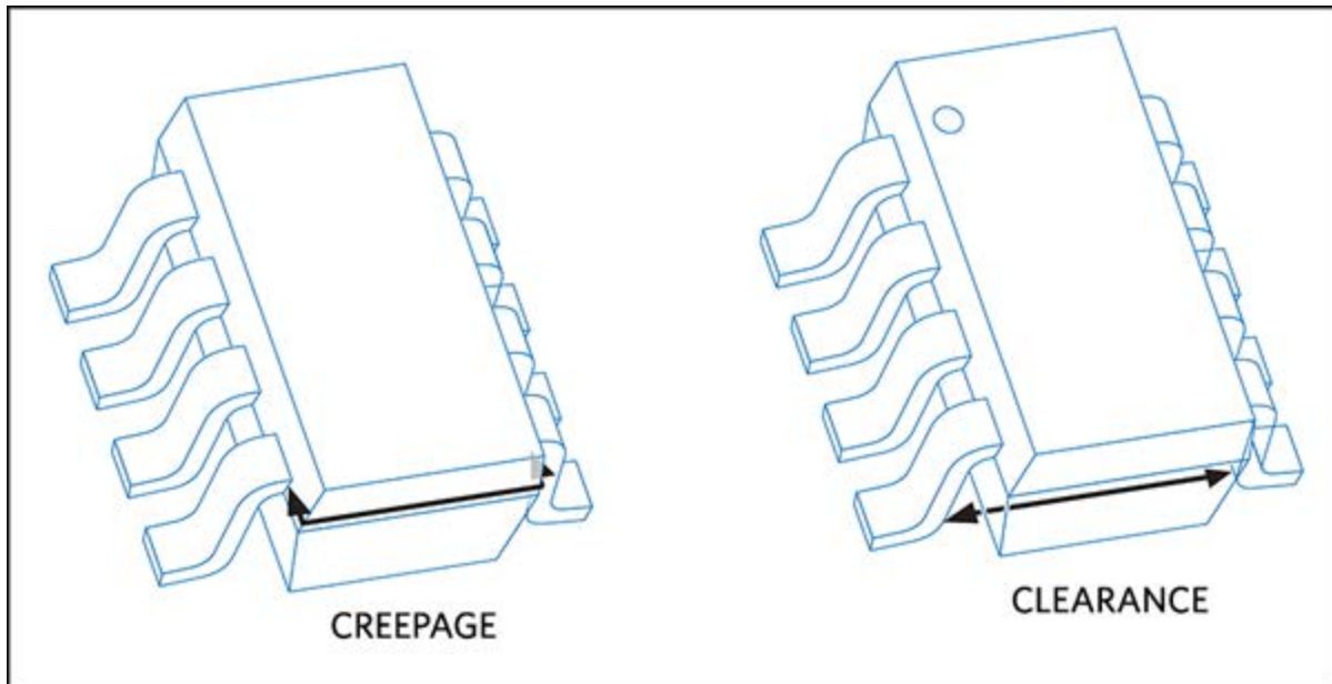
Figure 1. Creepage and clearance for semiconductor packages.
