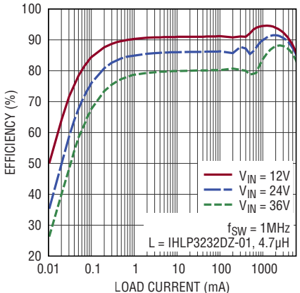
LT8640S Low Load Efficiency at 3.3V OUT
