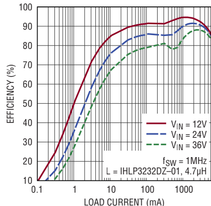
LT8643S Low Load Efficiency at 3.3V OUT
