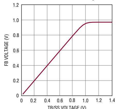
LT8640S Soft-Start Tracking
