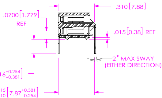
SECTION "D"- "D"
