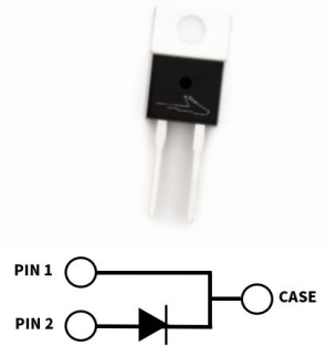
Package Types: TO-220-2 Marking: C4D08120A
