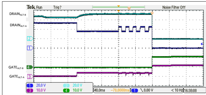
Figure 10-22. 4-Pair Single Signature 5-Finger Classification and Turn On
