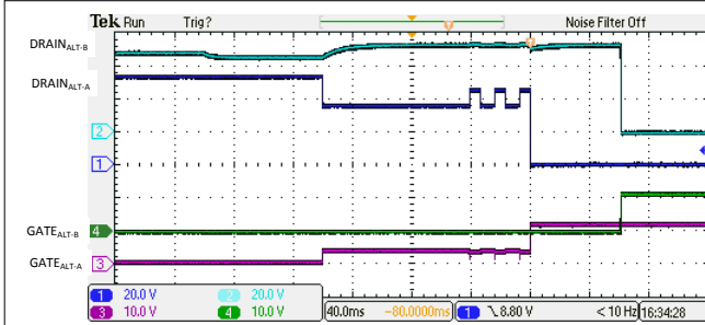
Figure 10-20. 4-Pair Single Signature 3-Finger Classification and Turn On
