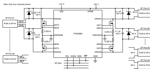
Simplified Schematic
