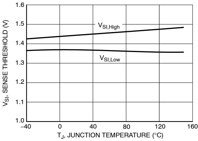
Figure 9. Sense Threshold vs. Junction Temperature
