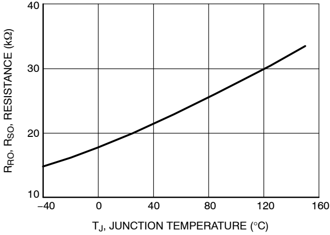
Figure 30. Resistance vs. Junction Temperature
