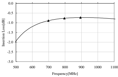
Insertion Loss
