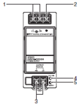
S8VS-12024 (120W)
