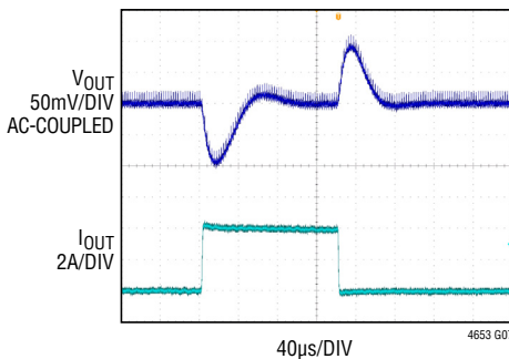
FIGURE 30 CIRCUIT, 48V IN , C INH = C D = 4.7µF, C OUT = 2 x 100µF, R FSET = N/A, R ISET = 66.5kΩ, C TH = 10nF, R TH = 604Ω, R EXTVCC = N/A, C EXTVCC = N/A, 2A to 4A LOAD STEP AT 2A/µs
