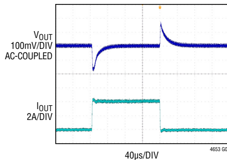
FIGURE 30 CIRCUIT, 48V IN , C INH = C D = 4.7µF, C OUT = 2 x 22µF, R FSET = 124k, R ISET = 240kΩ, C TH = 10nF, R TH = 562Ω, R EXTVCC = 49.9Ω, C EXTVCC = 1µF, 2A to 4A LOAD STEP AT 2A/µs
