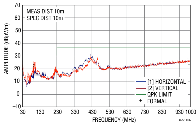
Figure 6. Radiated Emissions Scan of the LTM4653. Producing 12V OUT at 3A, from 58V IN . DC2327A Hardware. f_{SW} = 1.2\text{MHz} . Measured in a 10m Chamber. Peak Detect Method
