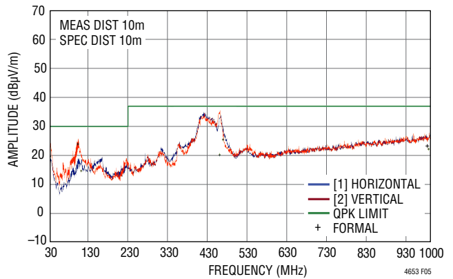
Figure 5. Radiated Emissions Scan of the LTM4653 Producing 24V OUT at 3.5A, from 48V IN . DC2327A Hardware. f_{SW} = 1.2\text{MHz} . Measured in a 10m Chamber. Peak Detect Method
