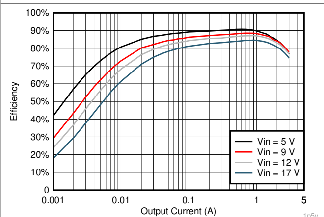
Figure 7-11. V_{OUT} = 1.5\text{ V} Efficiency, L = 1.5\ \mu\text{H}
