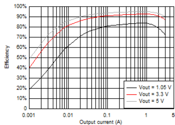
TPS563202S Efficiency
