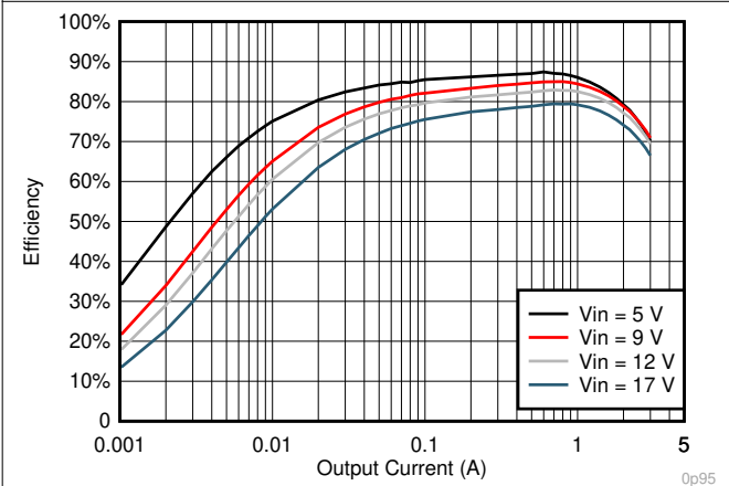
Figure 7-9. V_{OUT} = 0.95\text{ V} Efficiency, L = 1.2\ \mu\text{H}
