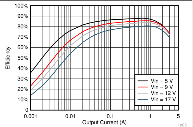
Figure 7-10. V_{OUT} = 1.05\text{ V} Efficiency, L = 1.2\ \mu\text{H}
