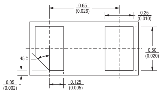
Model CDDFN2-T3.3B Bottom View
