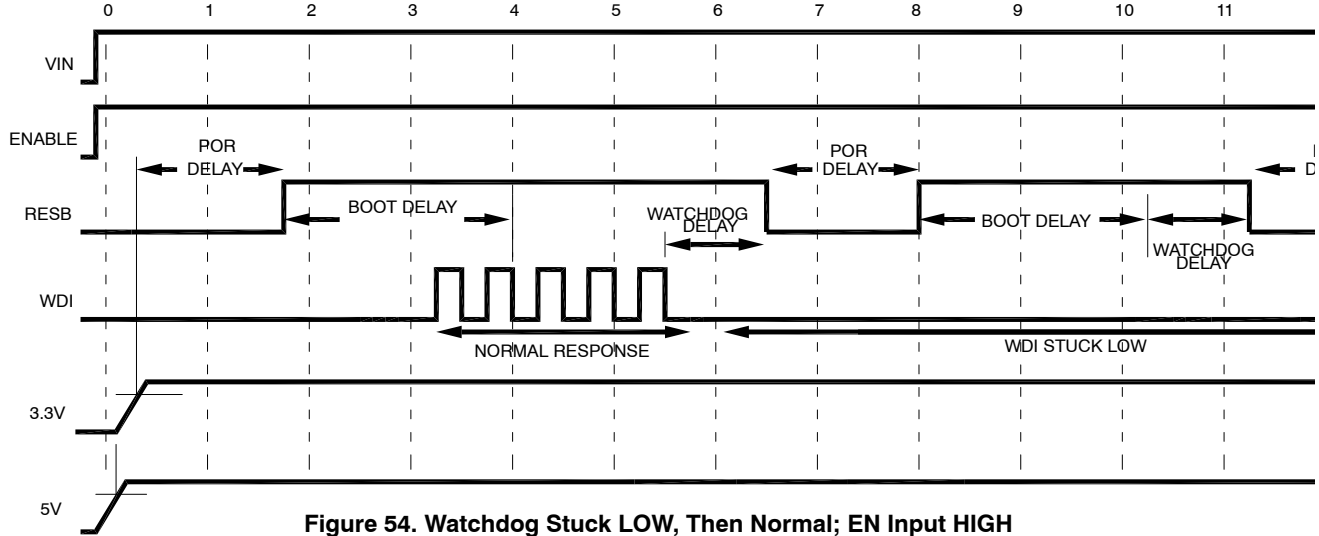
Figure 54. Watchdog Stuck LOW, Then Normal; EN Input HIGH
